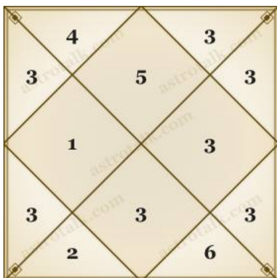
Saturn
